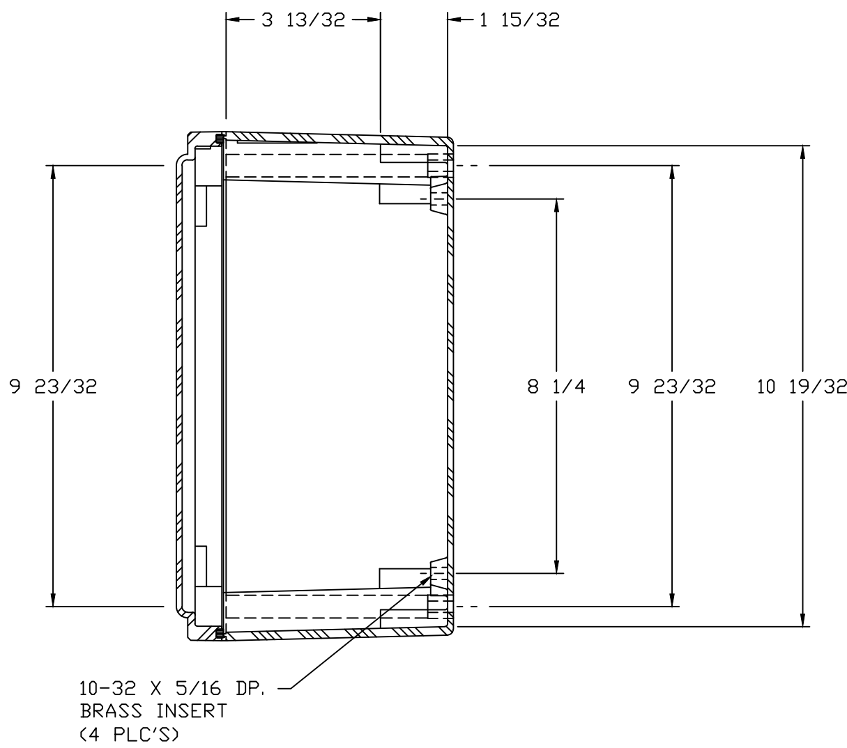
SECTION B-B
