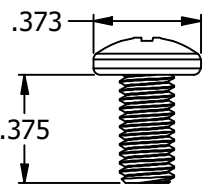
10-32 X 3/8" PHILLIPS PAN HEAD SS SCREW [4]
