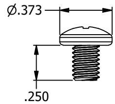
10-32 X 1/4" PHILLIPS PAN HEAD SS SCREW [4]
