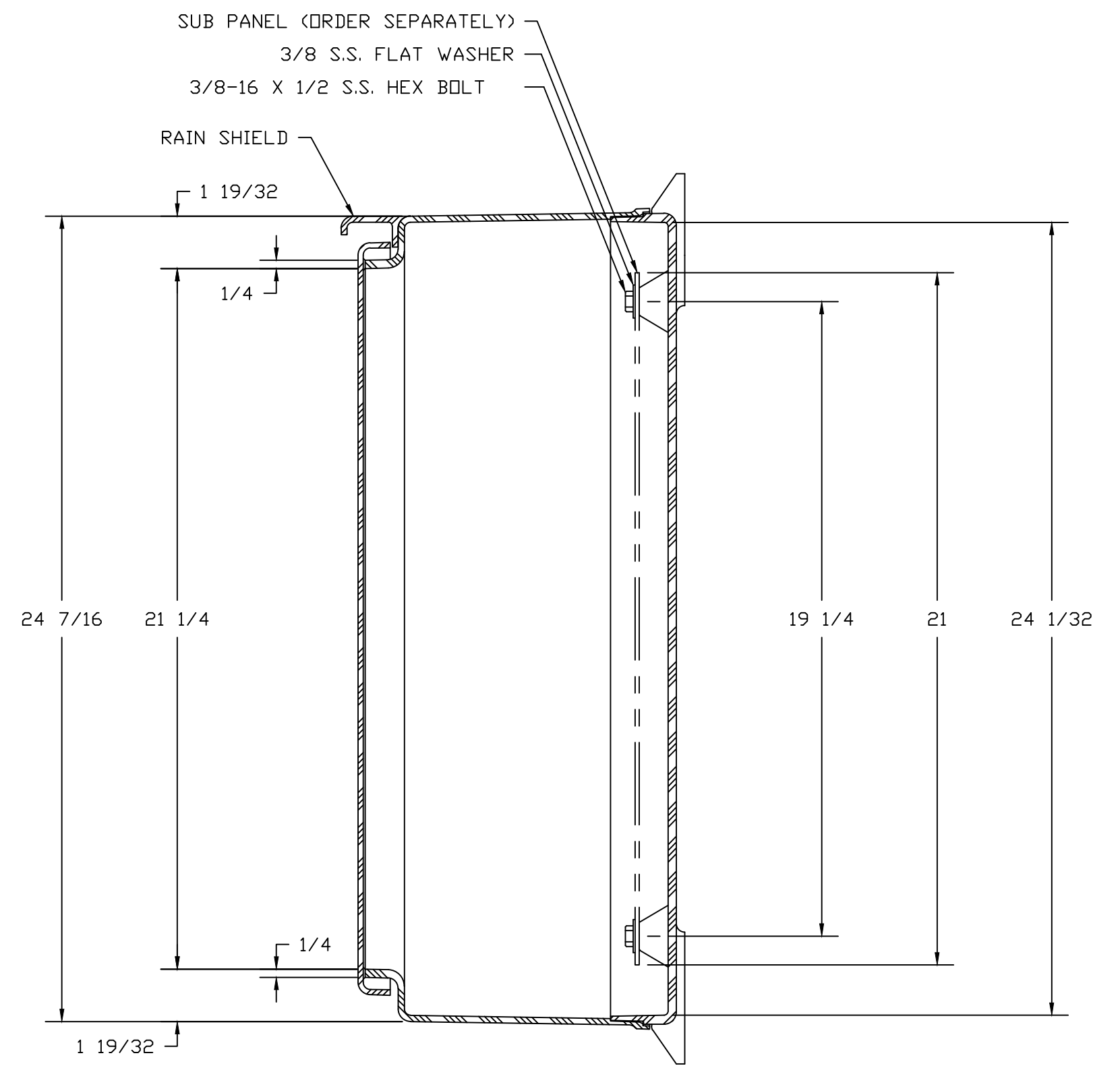
SECTION B-B
