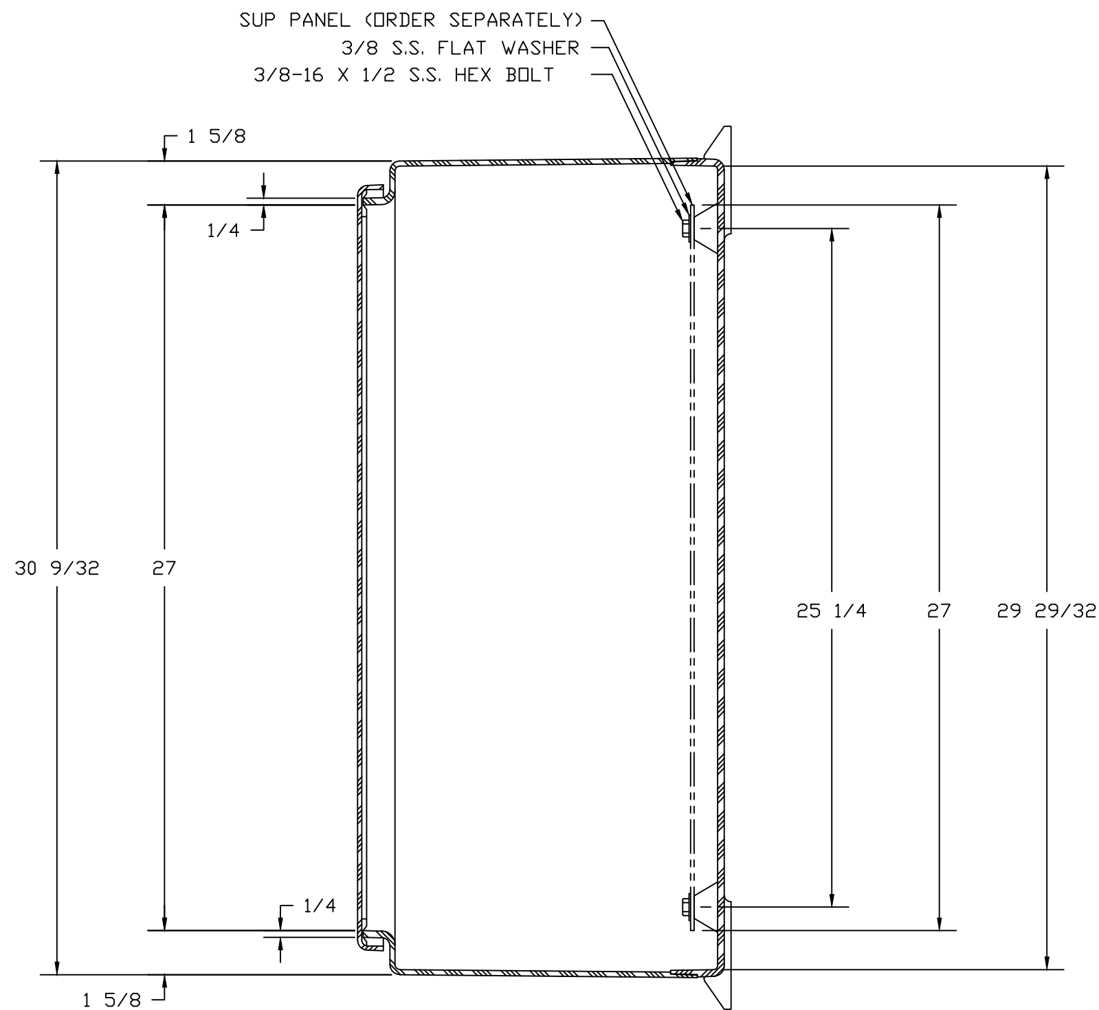
SECTION B-B
