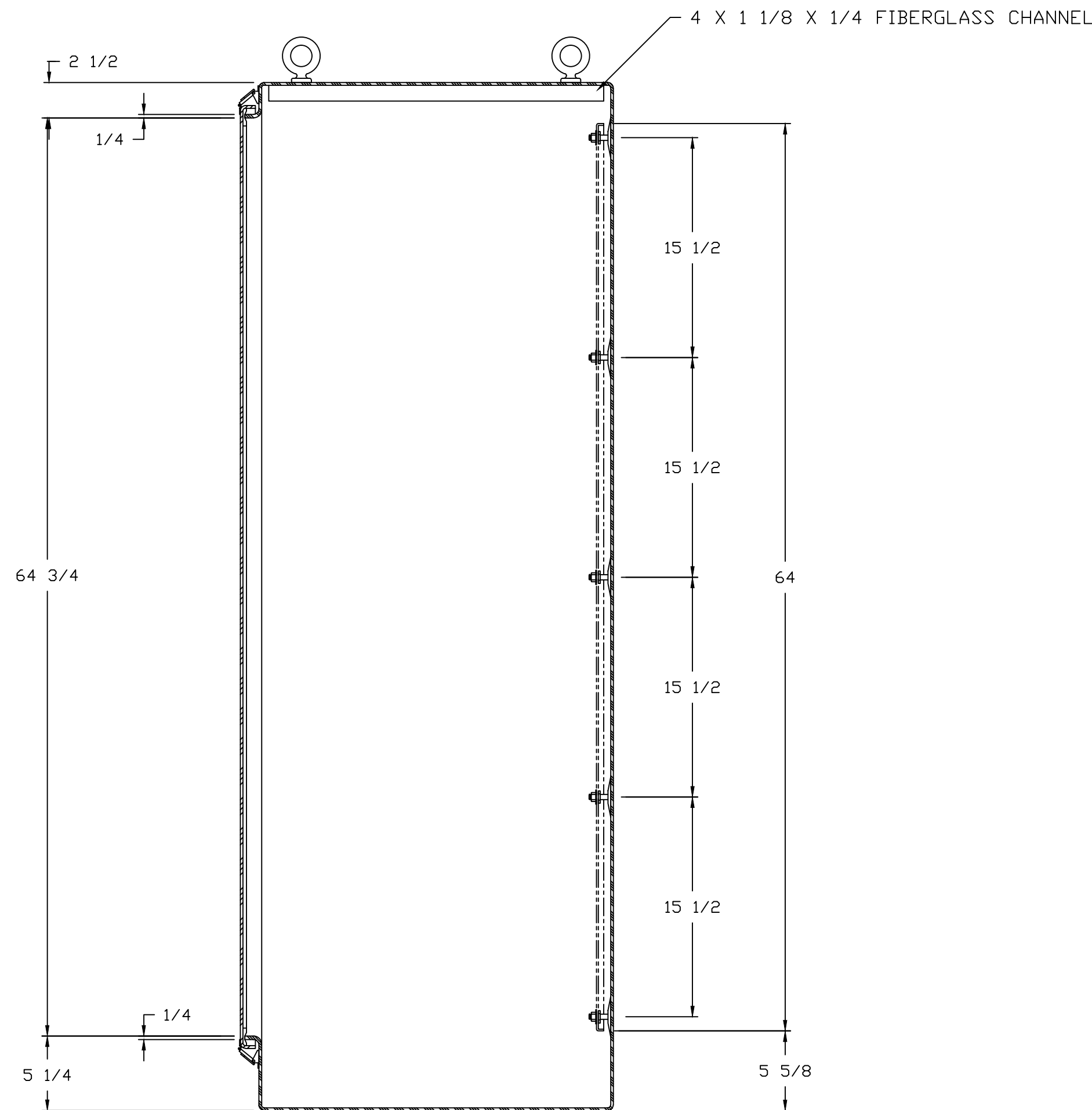
SECTION B-B
