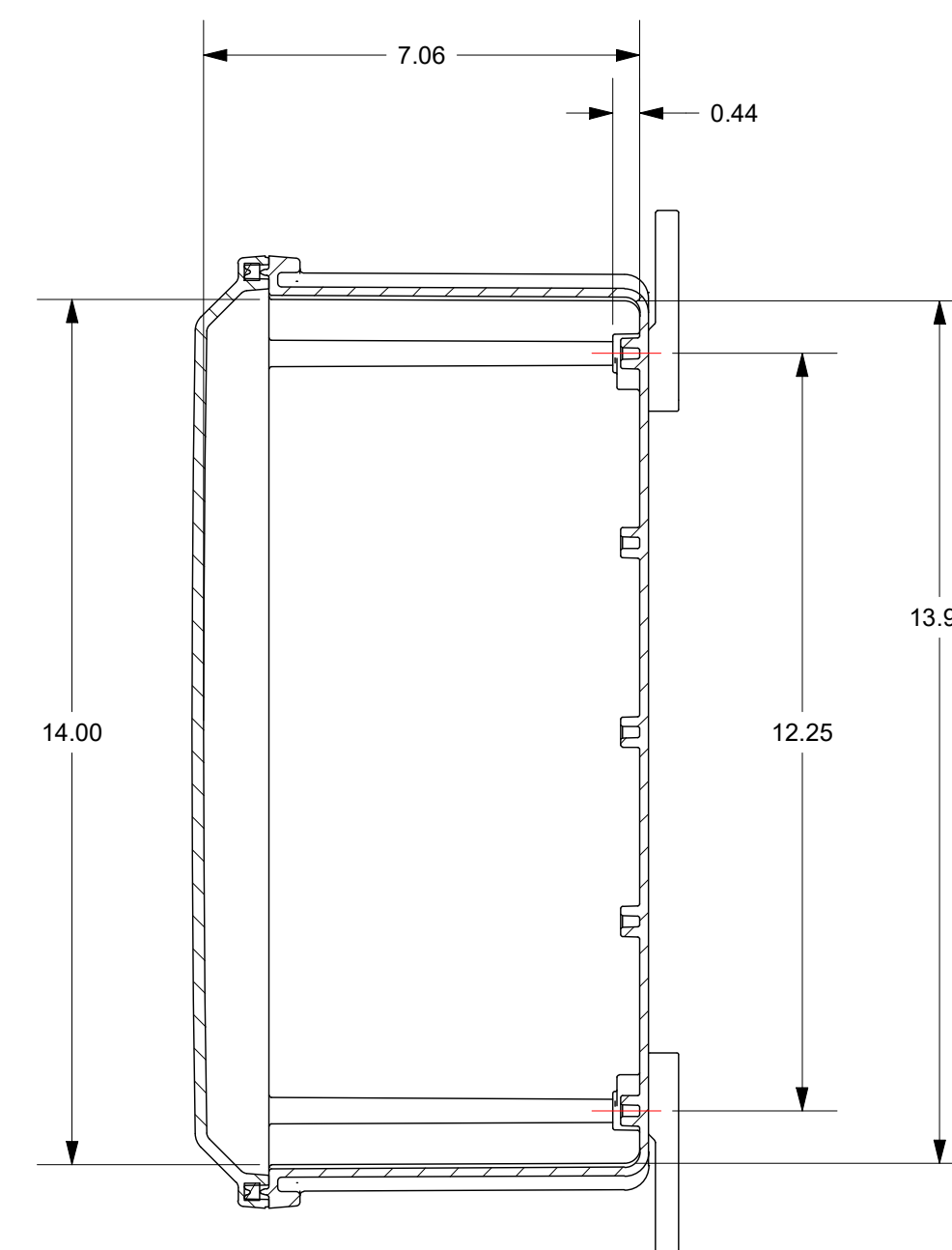
SECTION B-B
