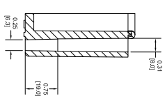
SECTION E-E SCALE 1:1
