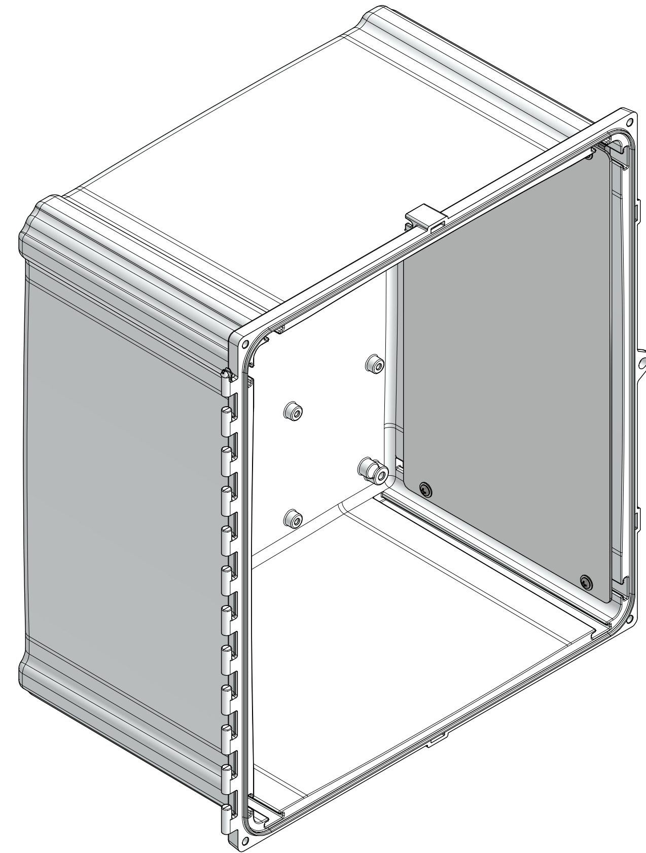
REF. VIEW - PANEL INSTALLED
