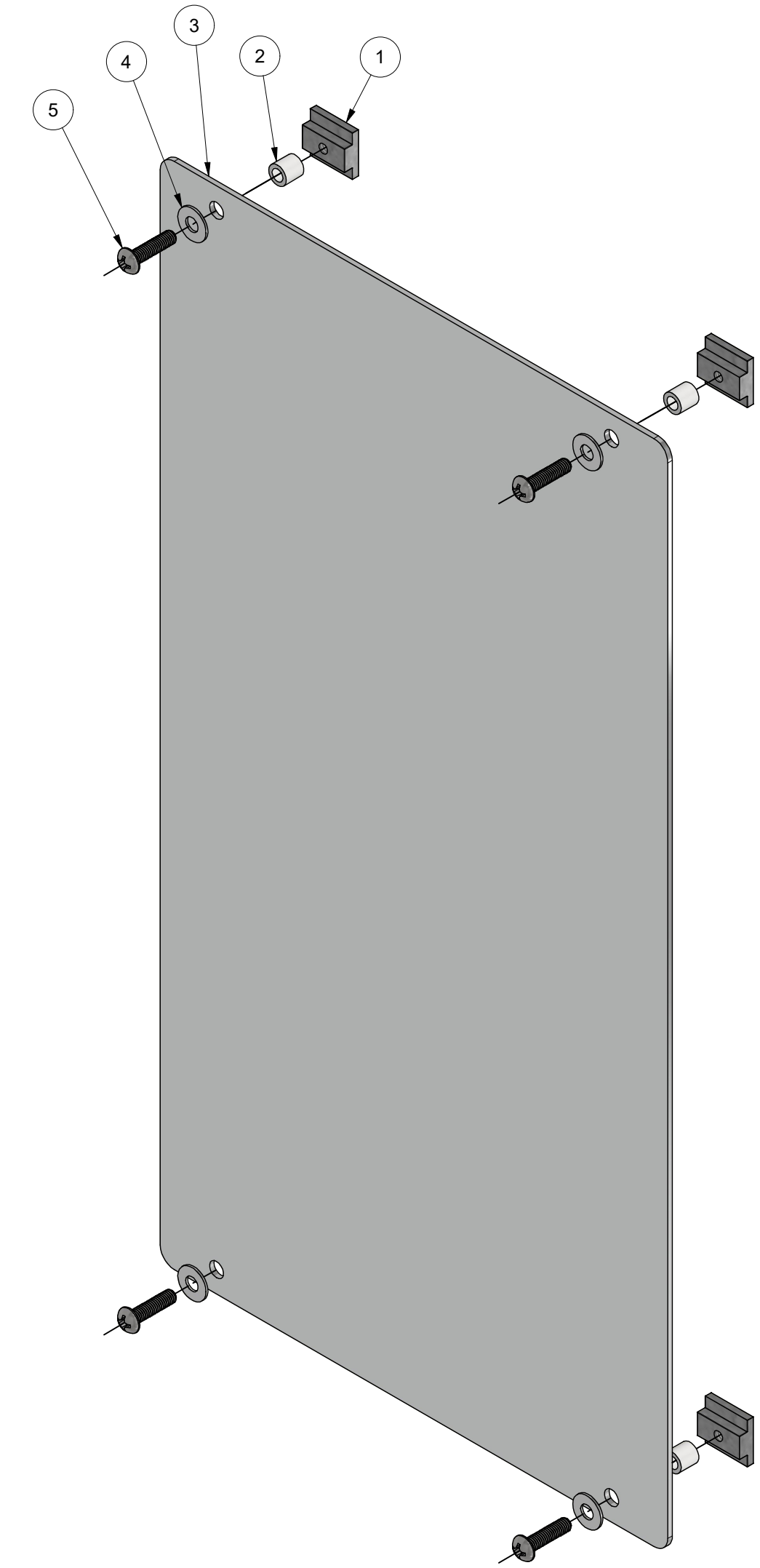
SIDE PANEL KIT
