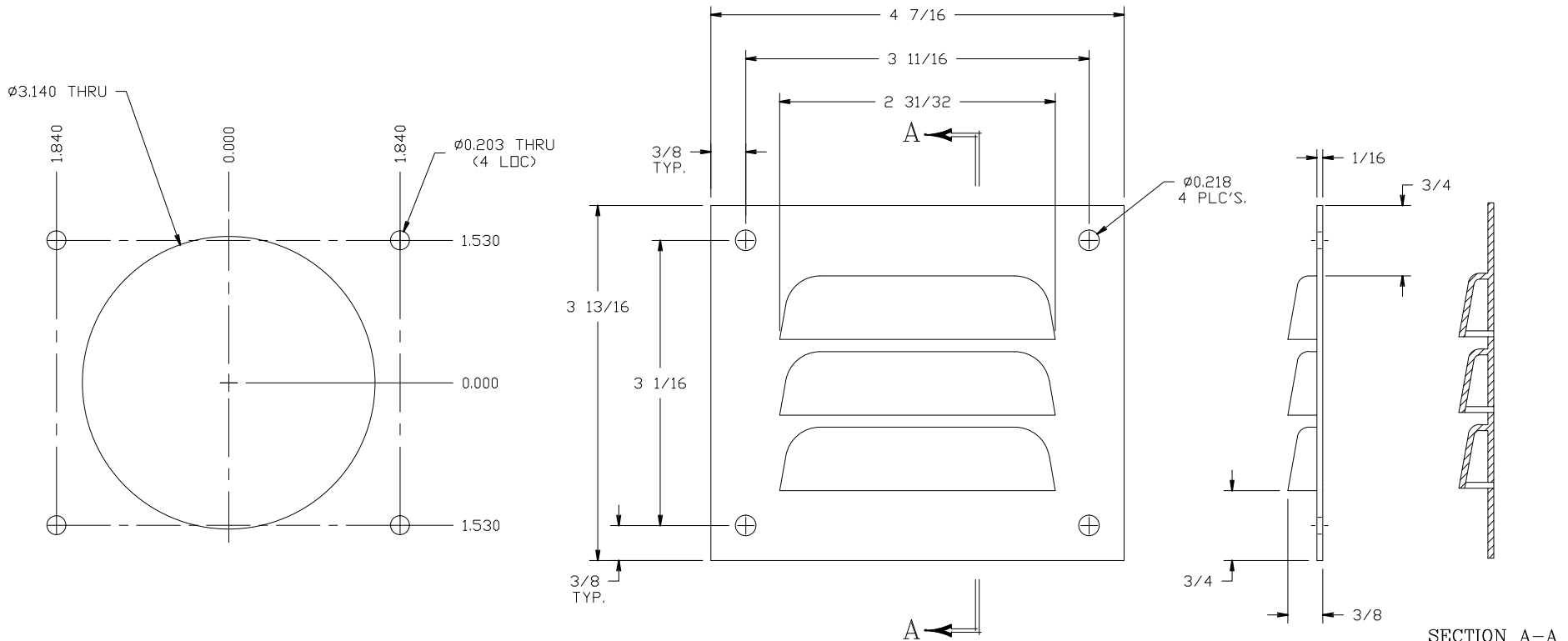
LOUVER PLATE CUT-OUT DETAIL
