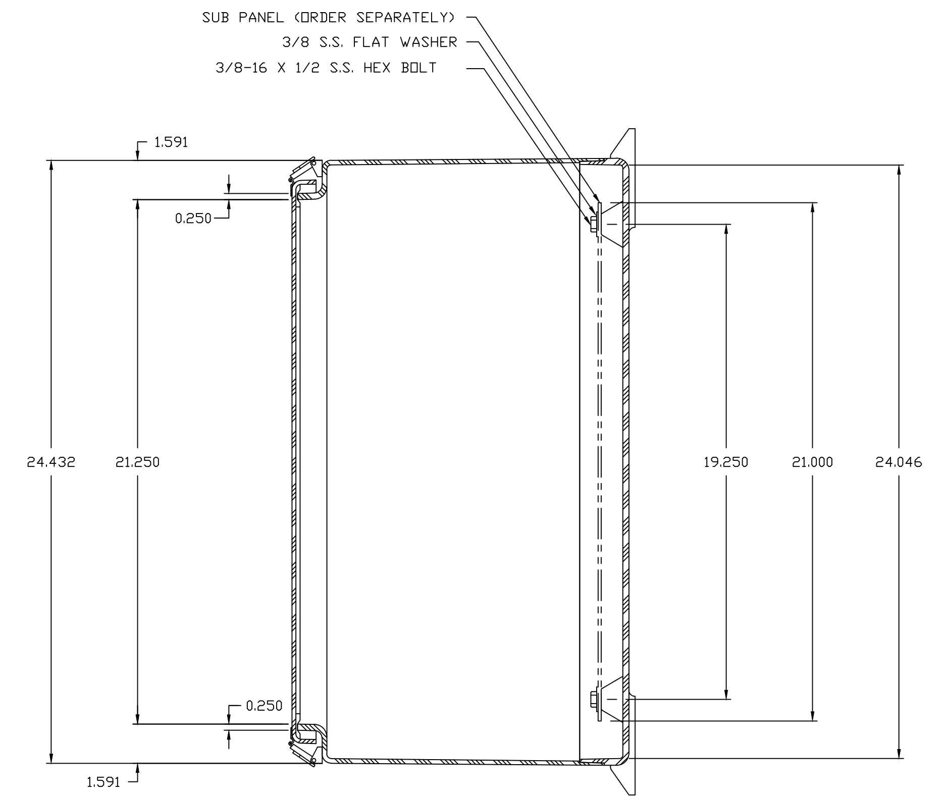
SECTION B-B
