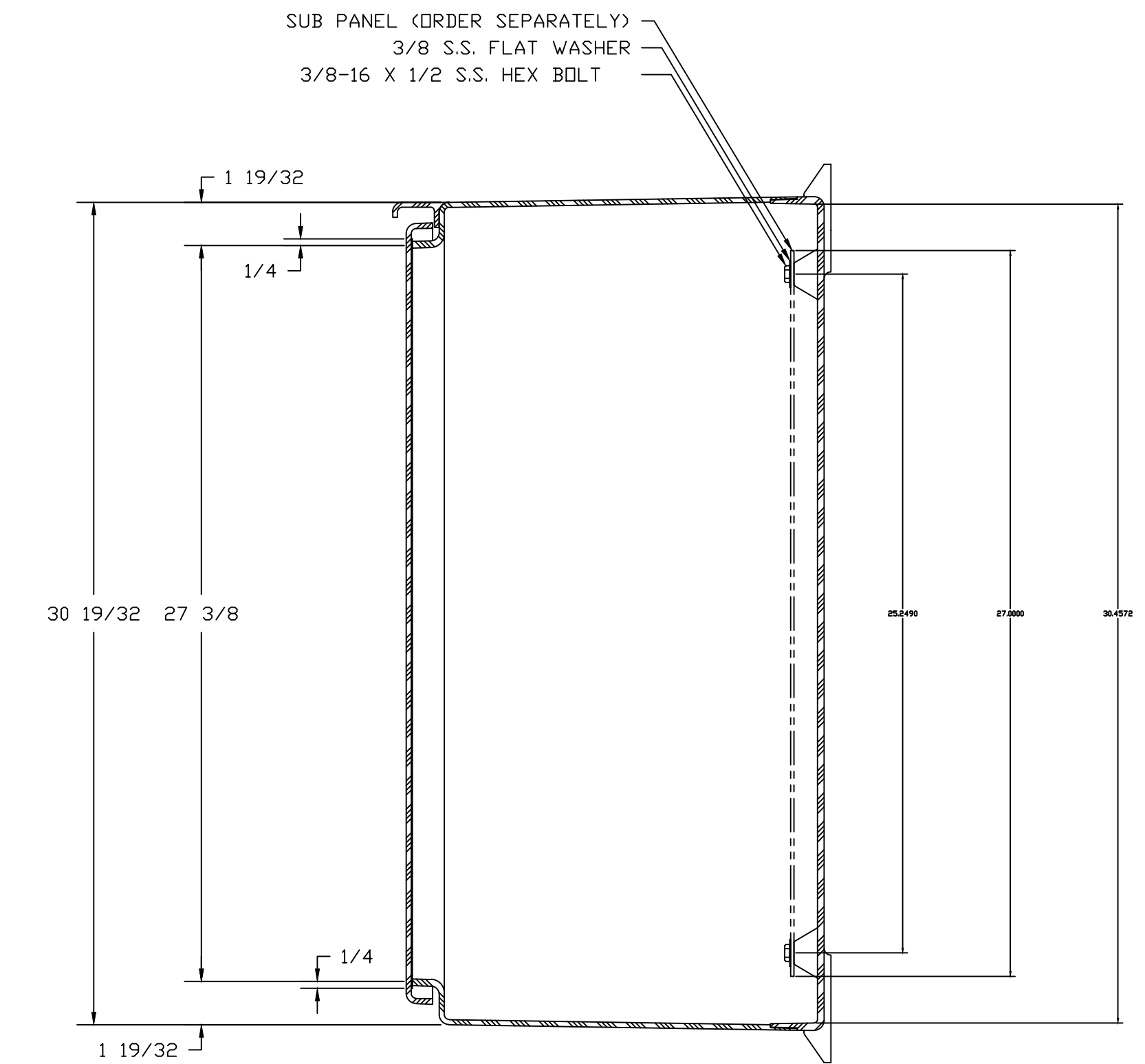
SECTION B-B
