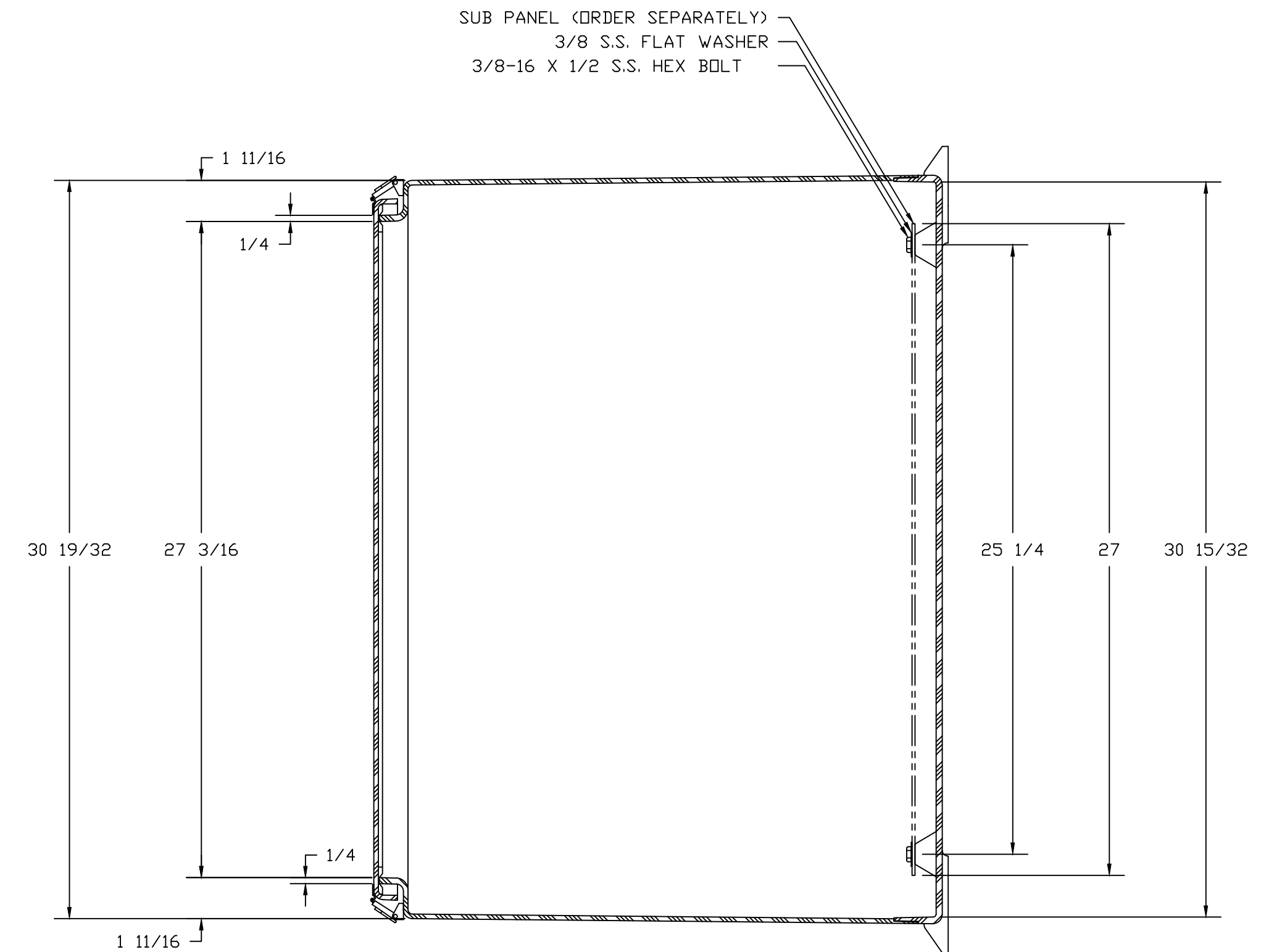
SECTION B-B
