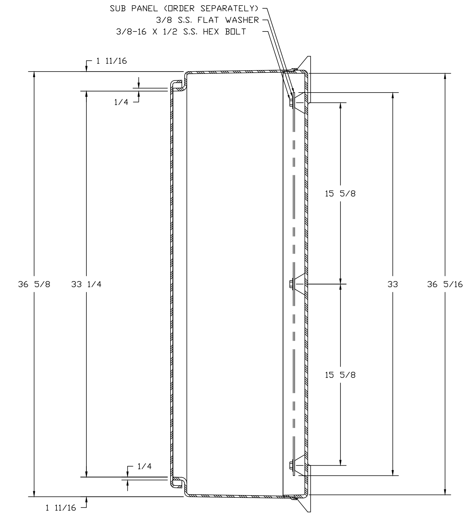
SECTION B-B
