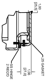
DETAIL A SCALE 1/2
