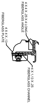
DETAIL B SCALE 1 / 4
