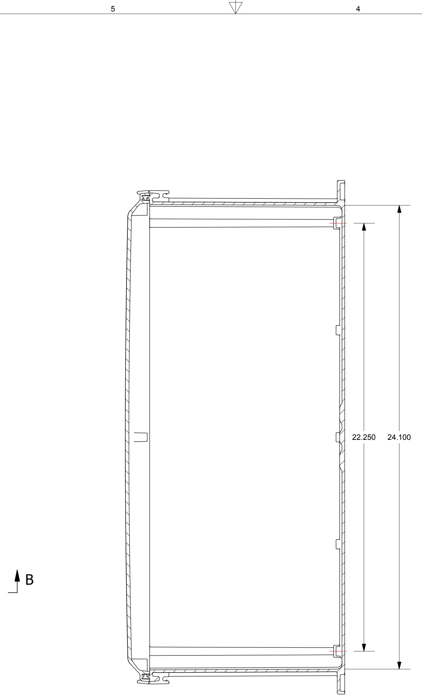
SECTION C-C
